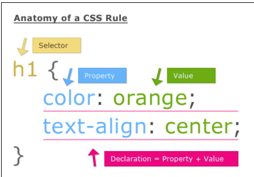
Figure 17: Anatomy of a CSS Rule
